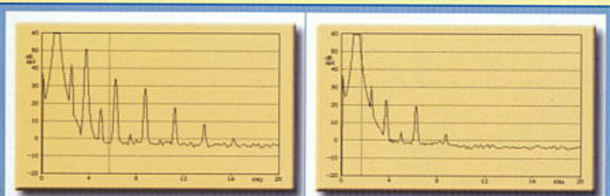
Conventional cabinet-FRQ=1250Hz
